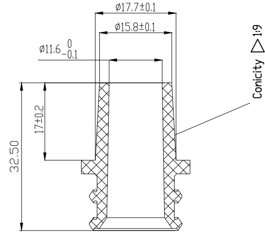
SECTION Q-Q
