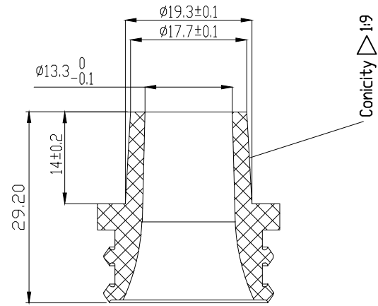
SECTION E-E
